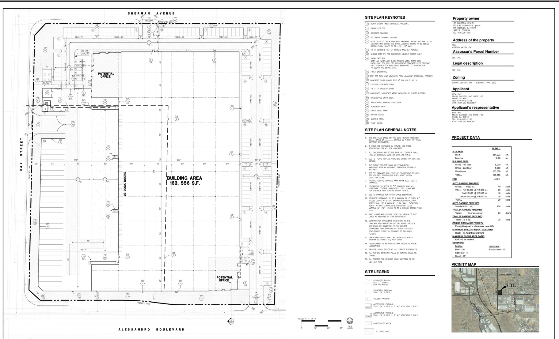
Figure 2.0-3 Site Plan The Moreno Valley Business Center Project
